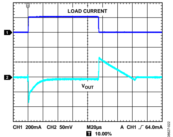
Figure 24. Load Transient Response, C_{IN} , C_{OUT} = 1\ \mu\text{F} , I_{LOAD} = 1\text{ mA} to 200\text{ mA}
